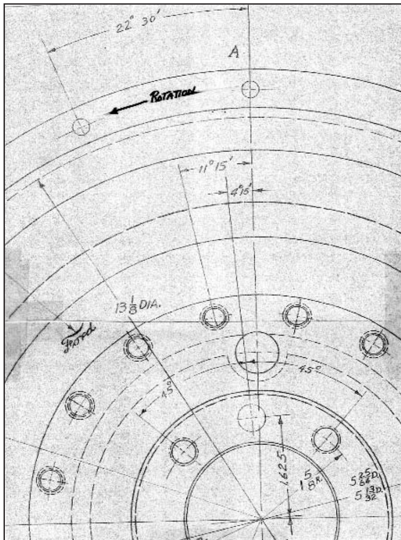
Figure 4 Flywheel Drawing T-701-C (partial) From the Research Center Collection at The Henry Ford Museum and Greenfield Village.
